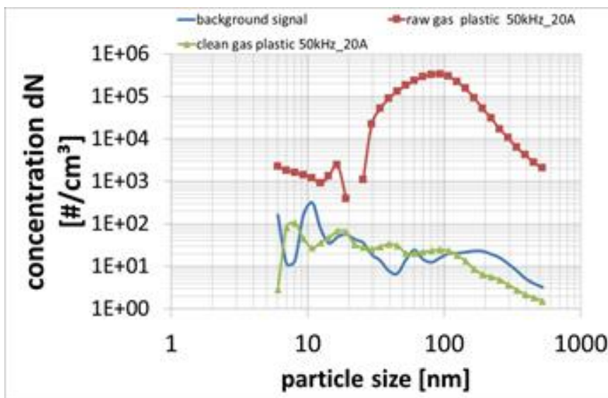
Figure 6: EEPs data of raw- and clean-gas during preparation of plastics with an ultra-fast laser. Clean gas was filtered by particle filter system LAS 260
